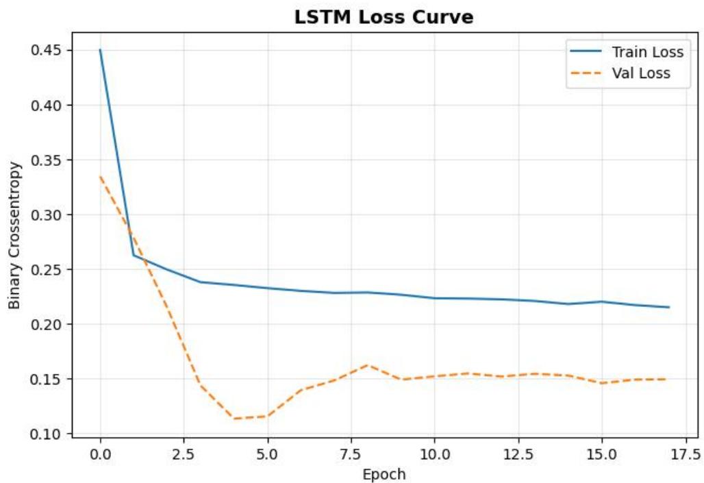
Figure 7: Loss curve of the LSTM model showing training and validation loss trends.
