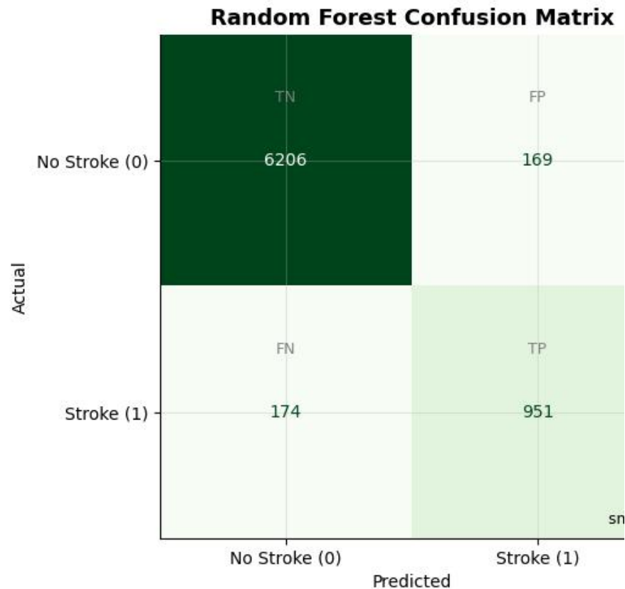
Figure 10: Confusion matrix of Random Forest model
