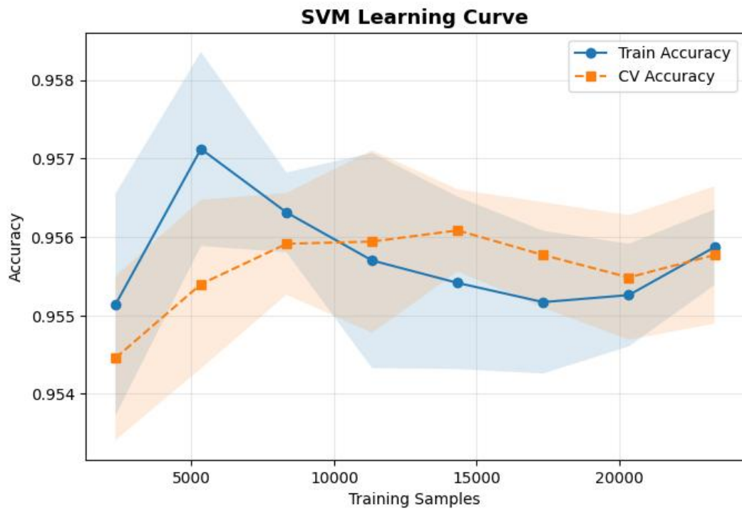
Figure 3: Learning curve of the SVM model showing training and validation accuracy convergence.
