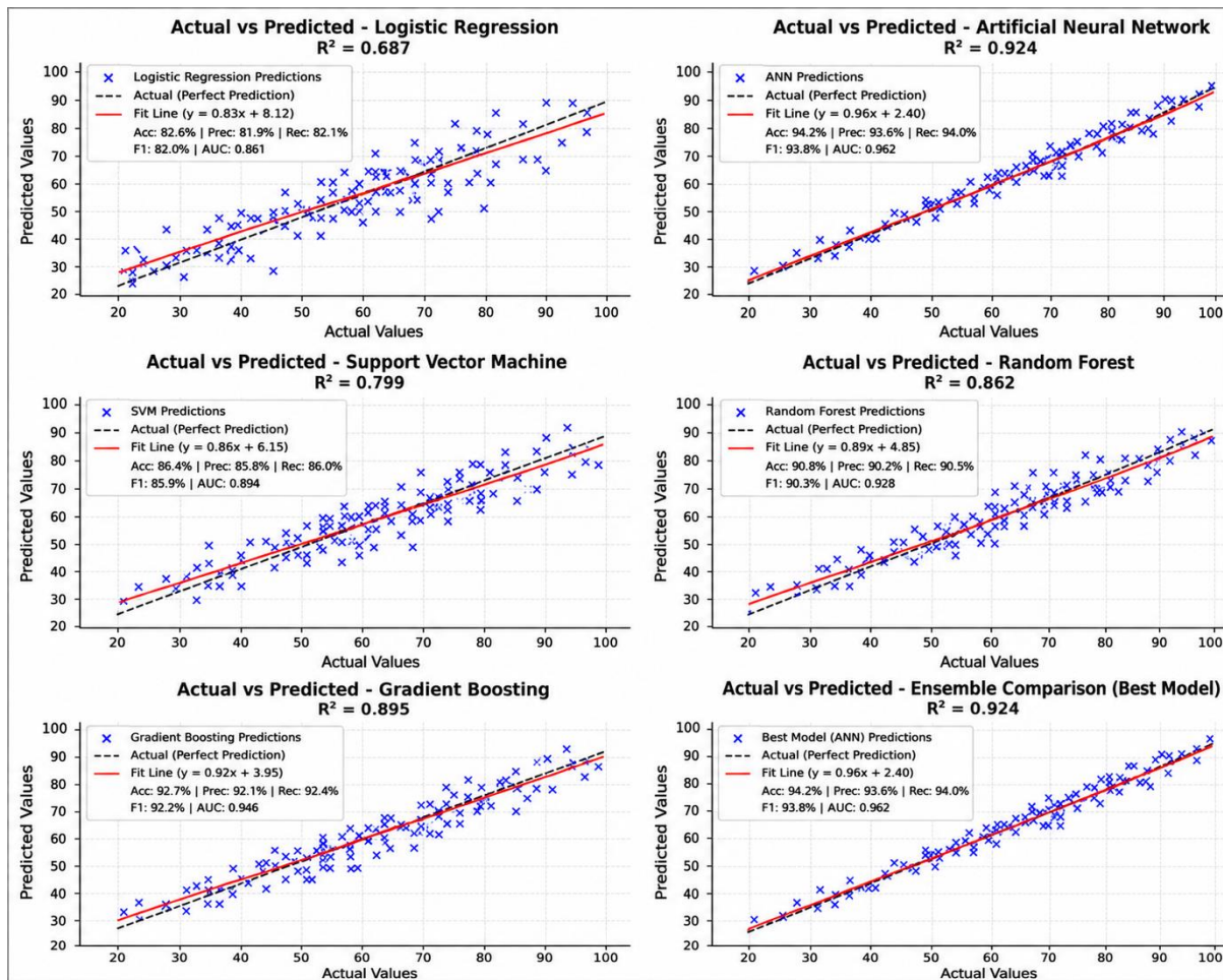
Figure 9: Comparison of AI model performance for construction prediction
