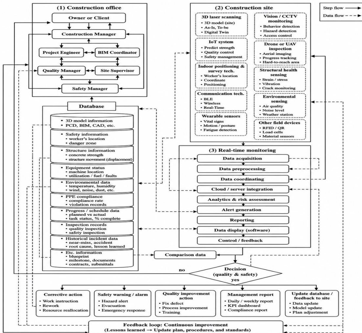
Figure 3: Smart construction intelligence framework for real-time quality, safety, and performance optimization.
