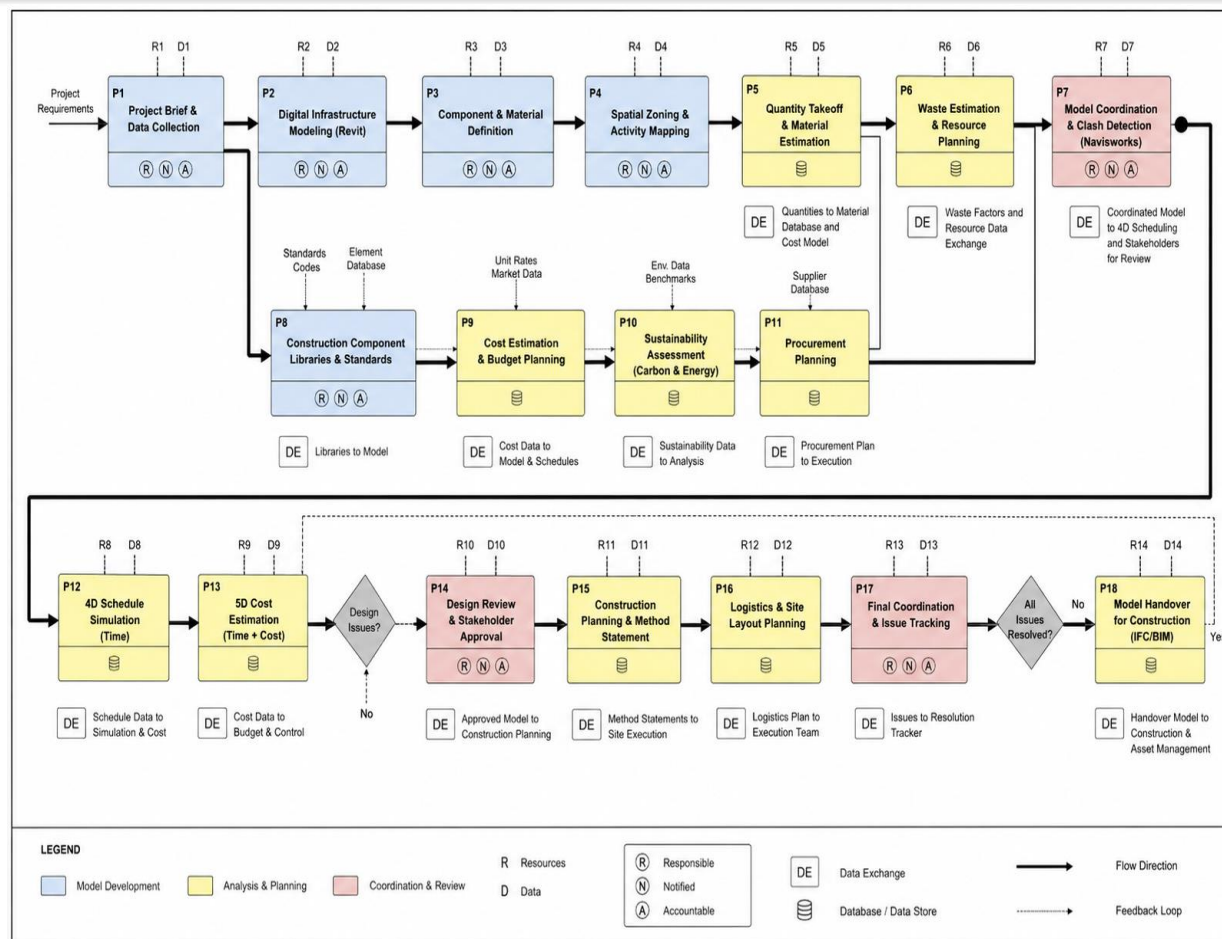
Figure 6: BIM-enabled construction planning and digital coordination workflow
