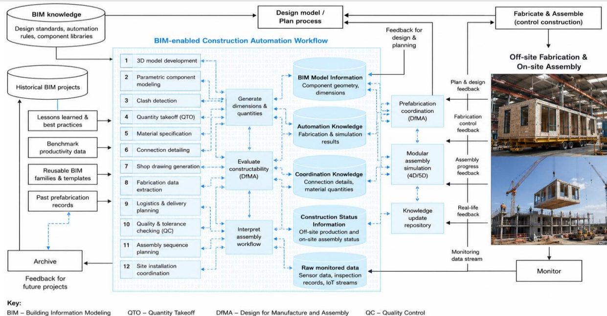
Figure 1: BIM-enabled construction automation workflow integrating design, prefabrication, assembly, monitoring, and feedback.
