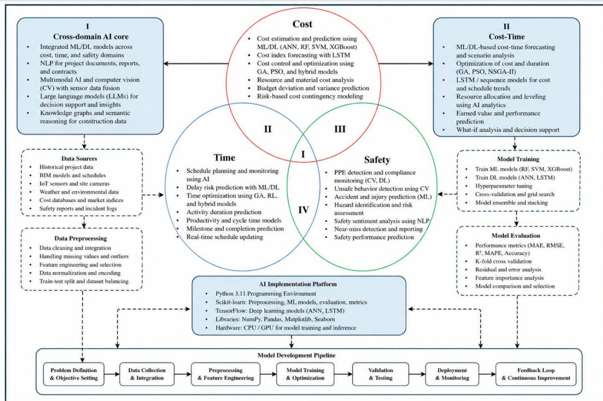
Figure 7: AI-based construction performance prediction workflow
