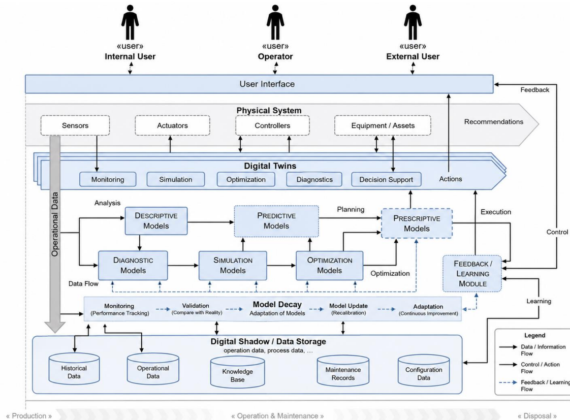
Figure 2: Digital twin and cyber-physical construction system architecture
