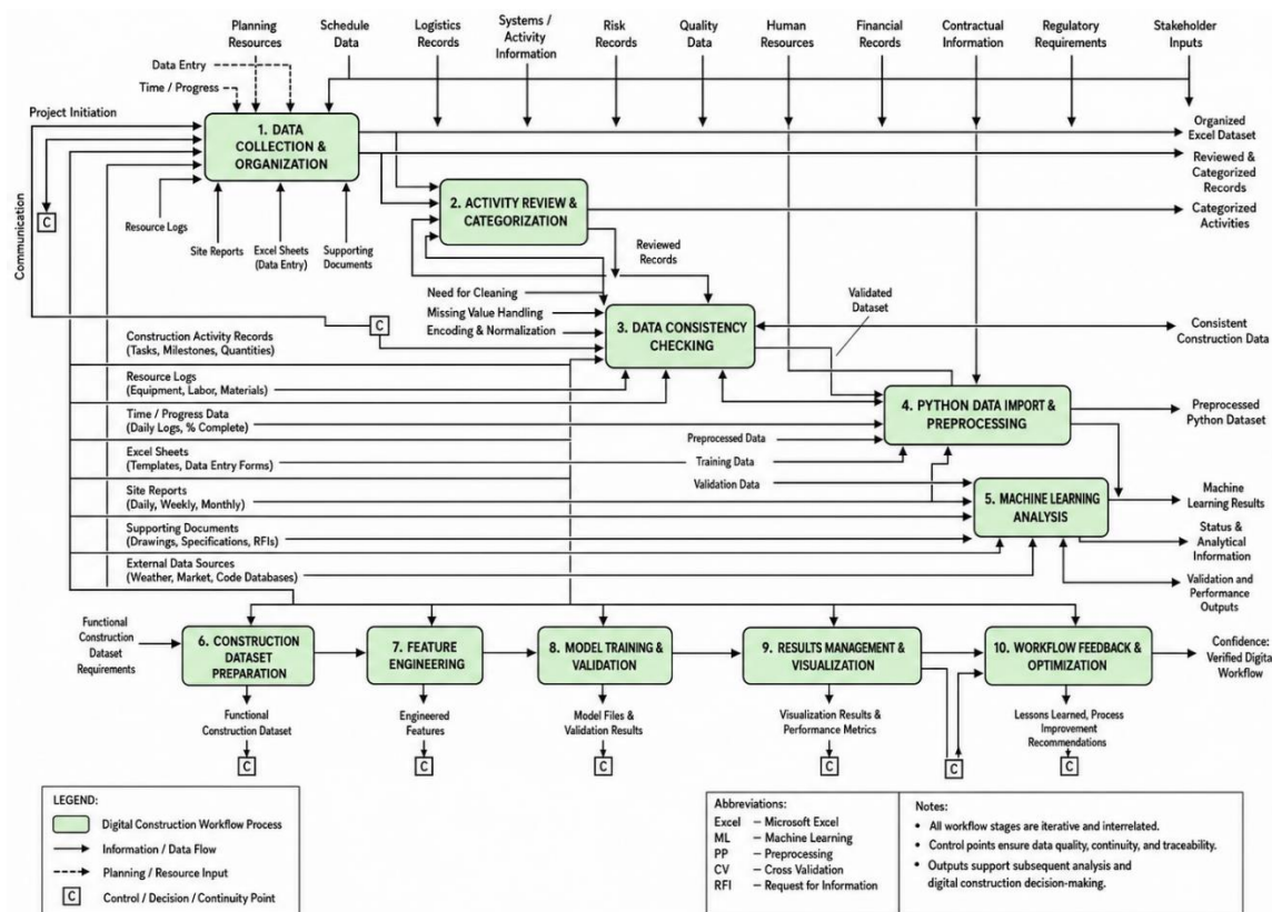
Figure 4: End-to-end data-driven Framework for construction analytics, machine learning validation, and digital workflow enhancement.
