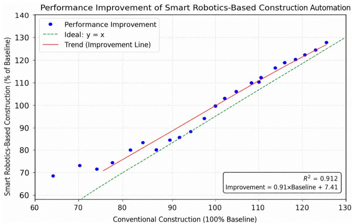
Figure 10: Performance improvement of smart robotics-based construction automation
