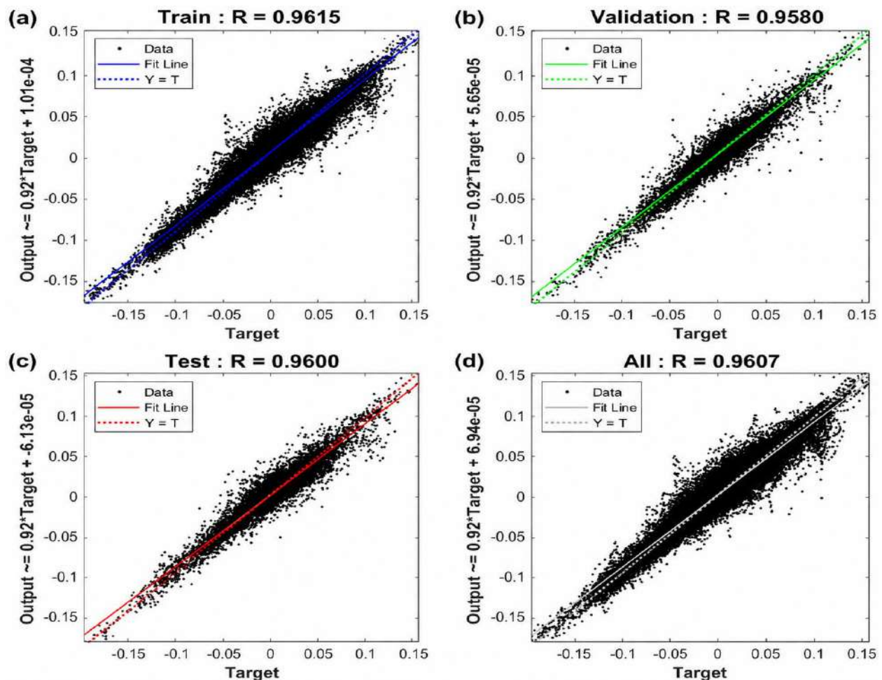
Figure 10: Regression performance between predicted outputs and targets for training, validation, testing, and combined datasets.
