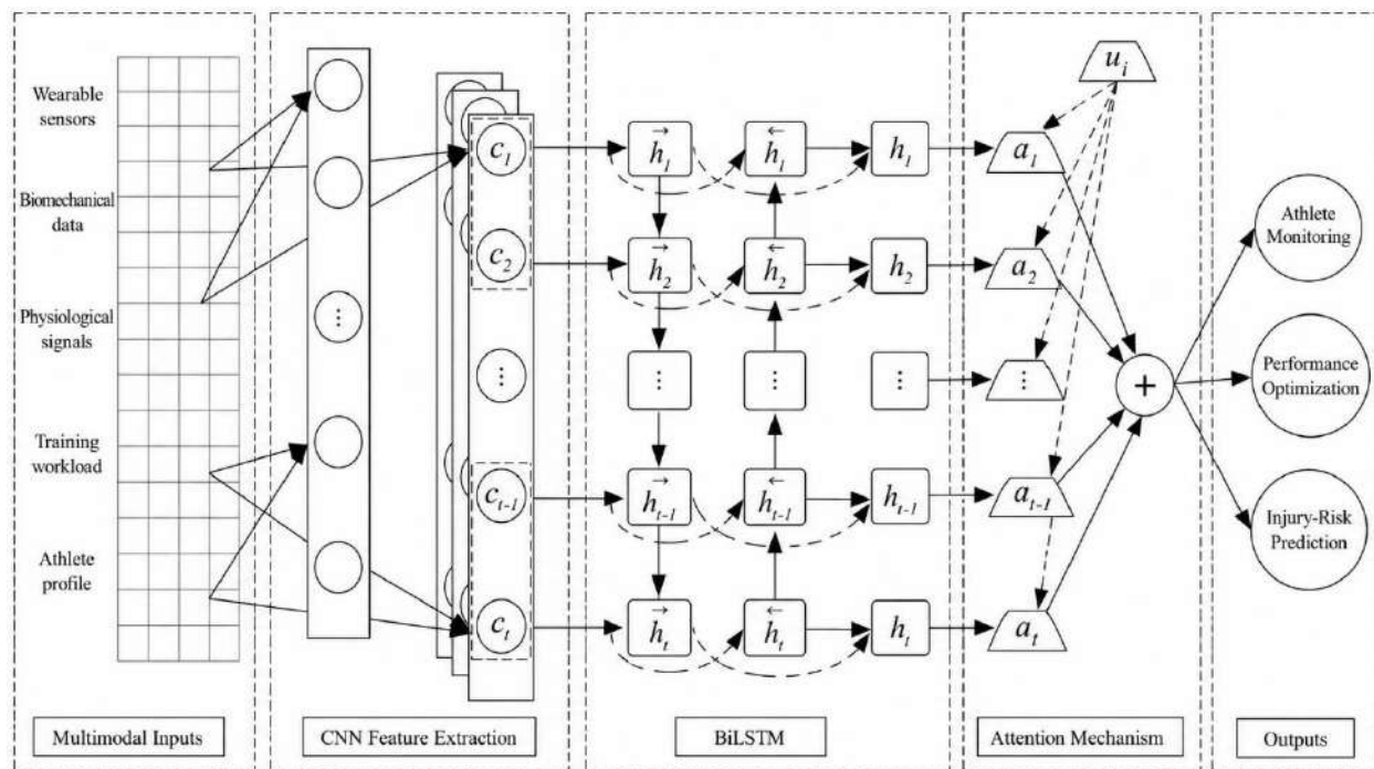
Figure 7: Proposed multimodal CNN-BiLSTM-attention architecture for athlete monitoring, performance optimization, and injury-risk prediction.
