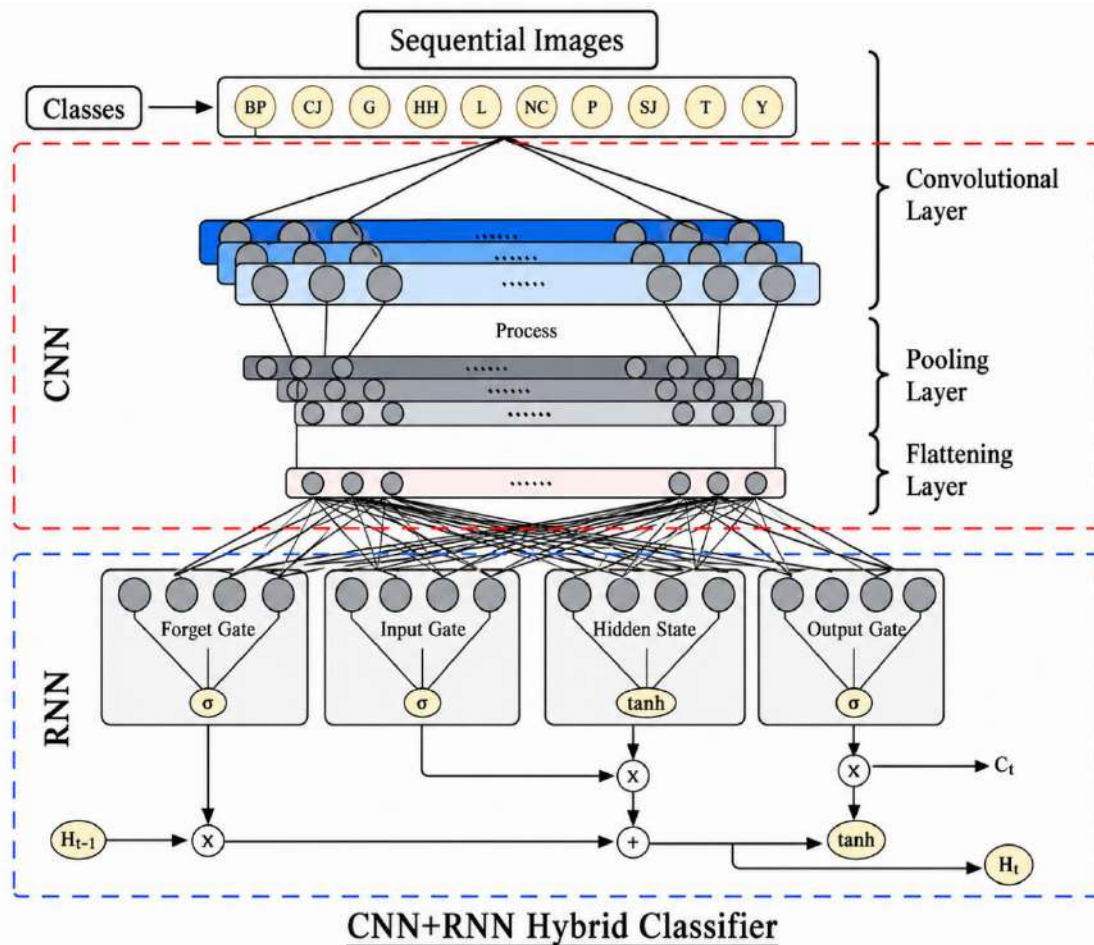
Figure 1: CNN-RNN hybrid architecture for sequential image classification.
