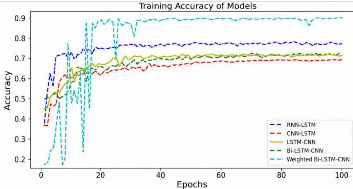
Figure 9: Training-accuracy comparison of recurrent and convolutional hybrid models across 100 epochs.
