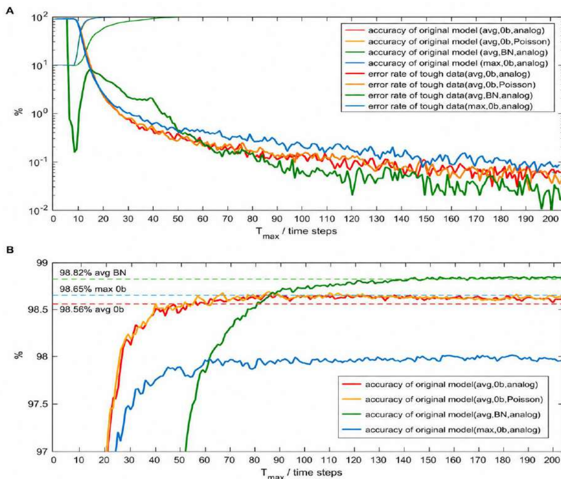
Figure 8: Model accuracy and tough-data error rates across increasing simulation time steps.
