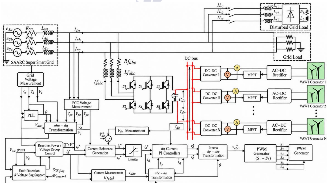
Figure 3: Grid-interfacing converter and voltage-support control pathway
