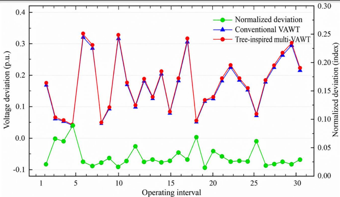
Figure 4: Normalized mean voltage deviation during annual operation
