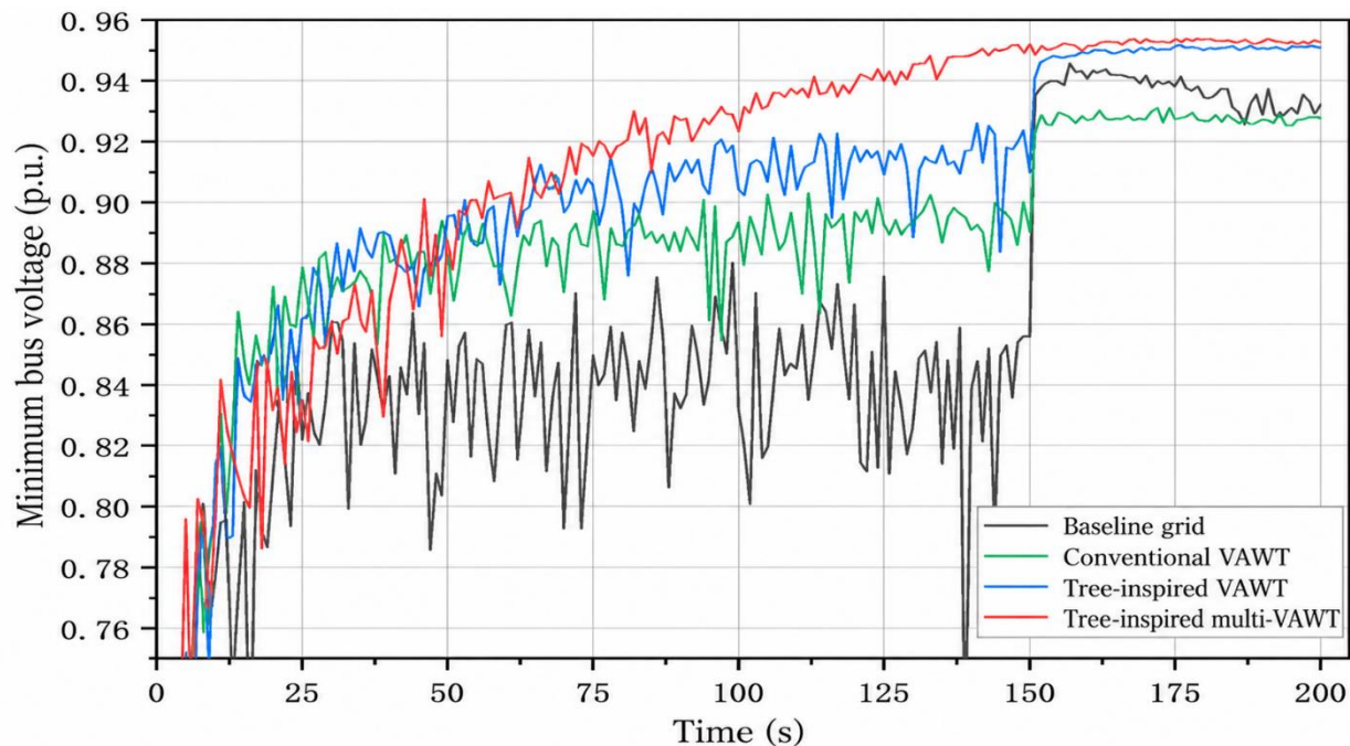
Figure 5: Minimum bus voltage during the most severe evaluated fault
