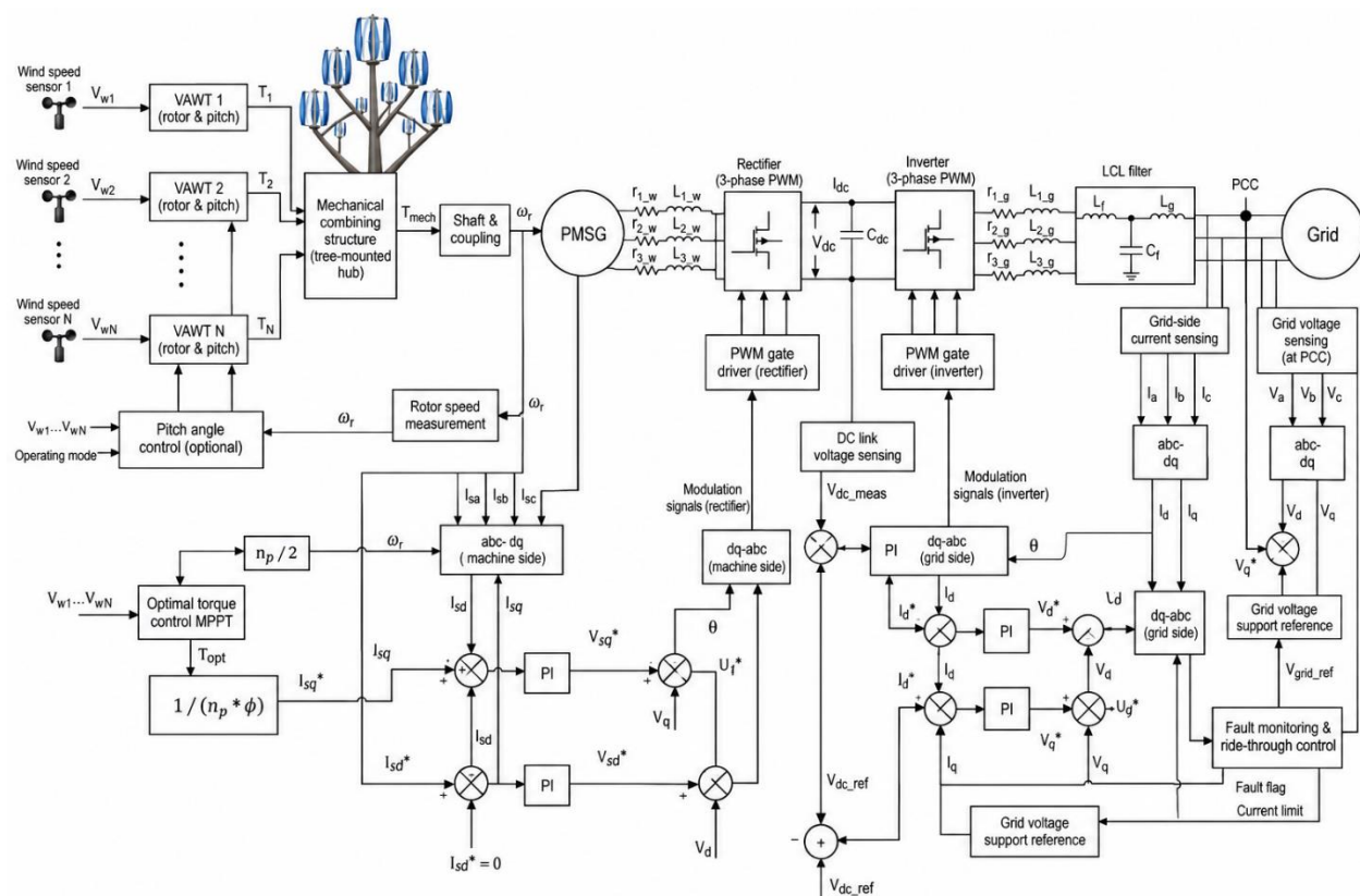
Figure 2: Tree-inspired multi-VAWT generation and grid-connection configuration
