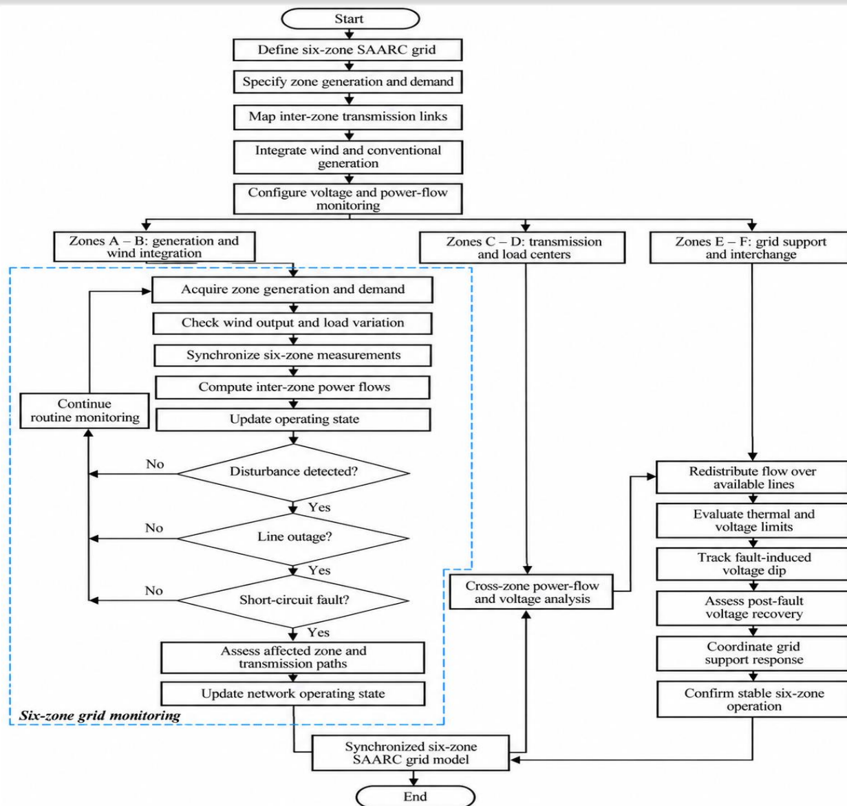
Figure 1: Functional arrangement of the six-zone SAARC super smart grid model
