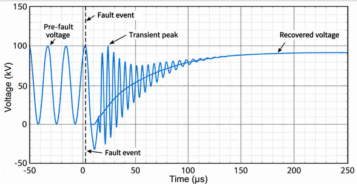
Figure 6: Post-fault voltage recovery time.
