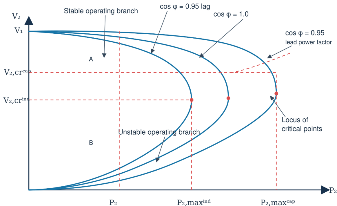
Figure 7: P-V curves showing the influence of power factor on voltage stability and loadability.
