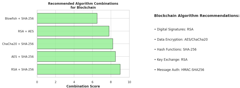
Figure 5: Recommended cryptographic algorithm combinations for blockchain layers (Data, Consensus, and Application) based on Composite Blockchain
