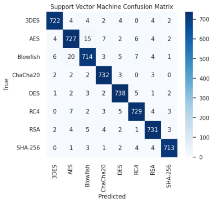
Figure 3: Confusion matrix for the Support Vector Machine (SVM) model, demonstrating classification performance across all cryptographic algorithm classes.
